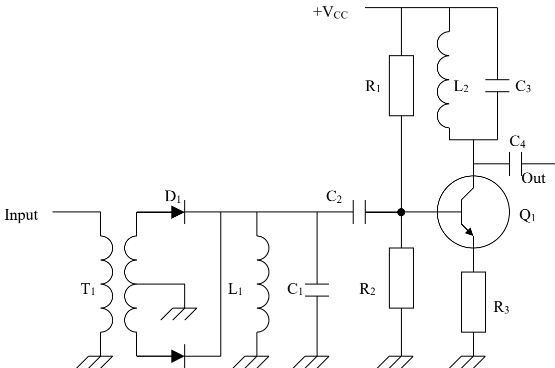
Frequency Doubler
