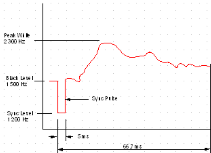
Monochrome SSTV signal
