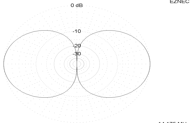
Radiation pattern of a dipole in free space
